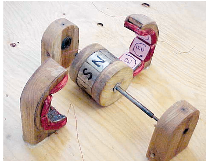
An exploded view shows the armature, stator, and pillow blocks ready to assemble into an alternator.
