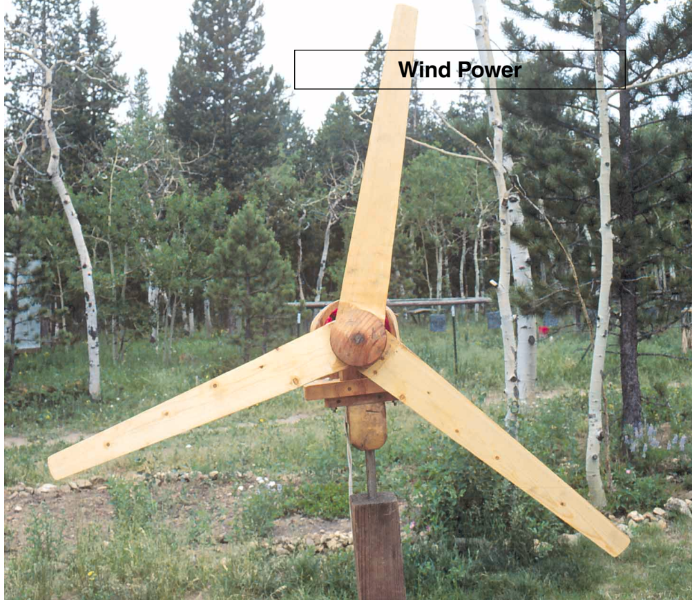
The Wood 103 has three, 2 foot, hand-carved blades, creating a swept area of 12.5 square feet.
