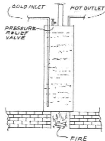
Figure 2. Water tank heated directly by fire.
