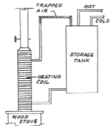
Figure 5. Trapped air in shaded area of pipe will prevent water from flowing.
