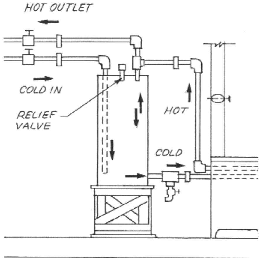
Figure 4. A properly plumbed system.
