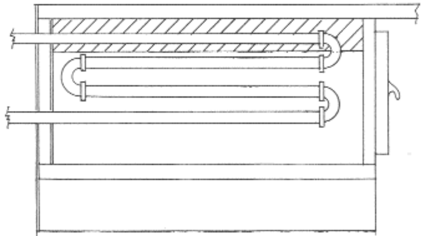
Figure 3. Cast iron pipe arrangement inside a firebox.
