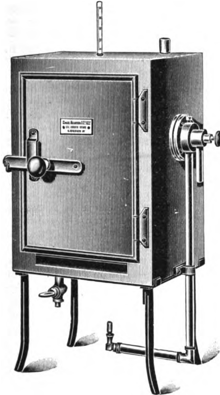
FIG. 156.—Paraffin oven.
