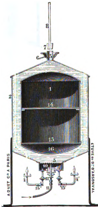
FIG. 52.—D'Arsonval's incubator in section.
