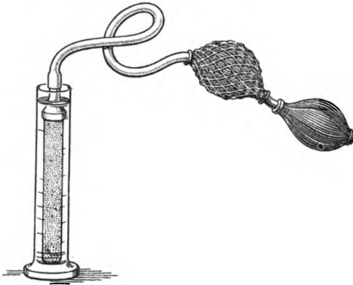
FIG. 12.—Method of testing a porcelain filter.
