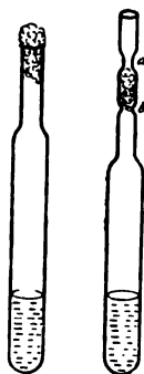
FIG. 95.—Esmarch's tubes applied to anaerobic cultivation.
