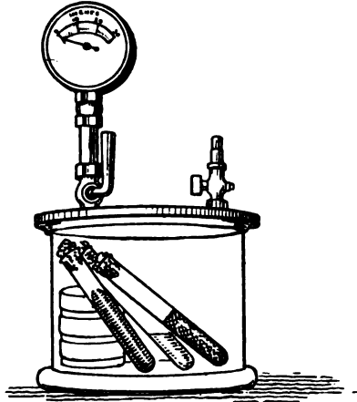
FIG. 97.—Tretróp's apparatus, in which to grow anaërobic cultures.
