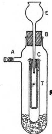
FIG. 29.—Laboratory bougie—Martin's arrangement.
