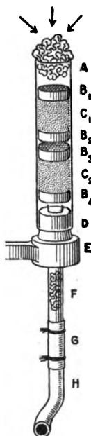
FIG. 412.—Petri's sand filter for the examination of air.
