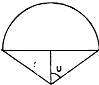
FIG. 108.—Numerical aperture.
