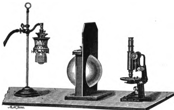
FIG. 111.—Illumination with an inverted incandescent gas burner.
