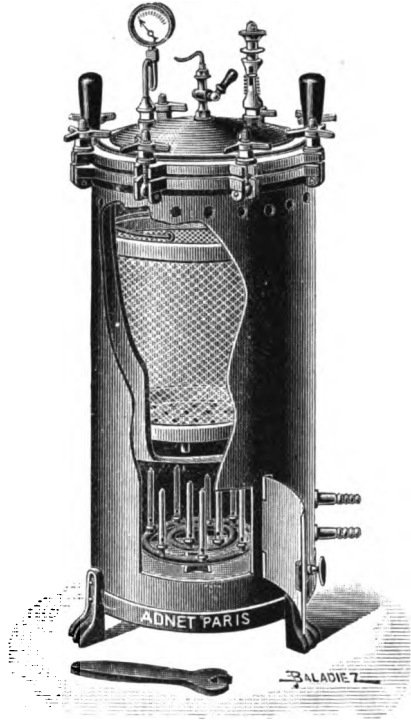
FIG. 6.—Chamberland's autoclave.
